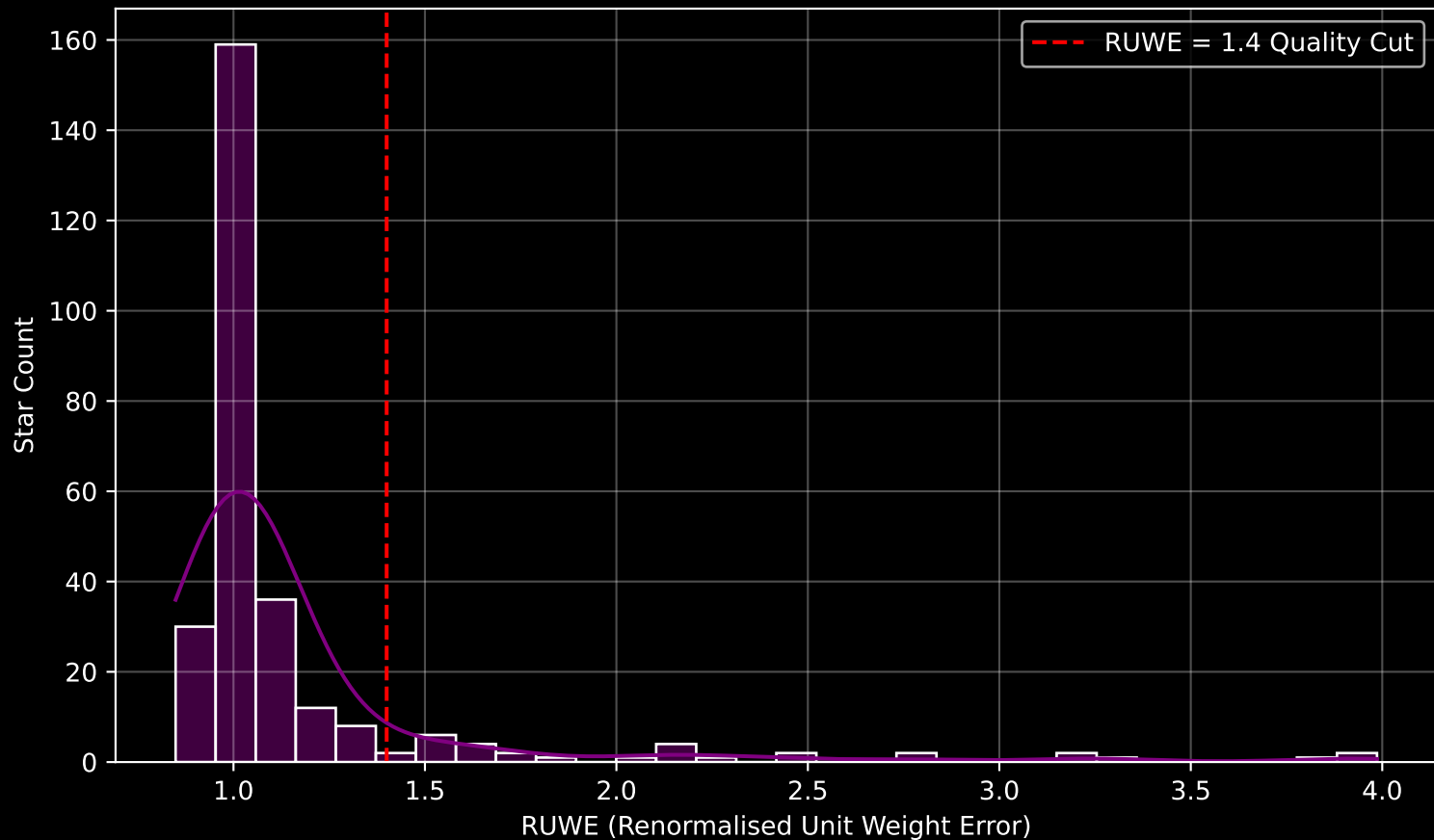
GALAH DR4 Field [647] RUWE Distribution (n= 276)
