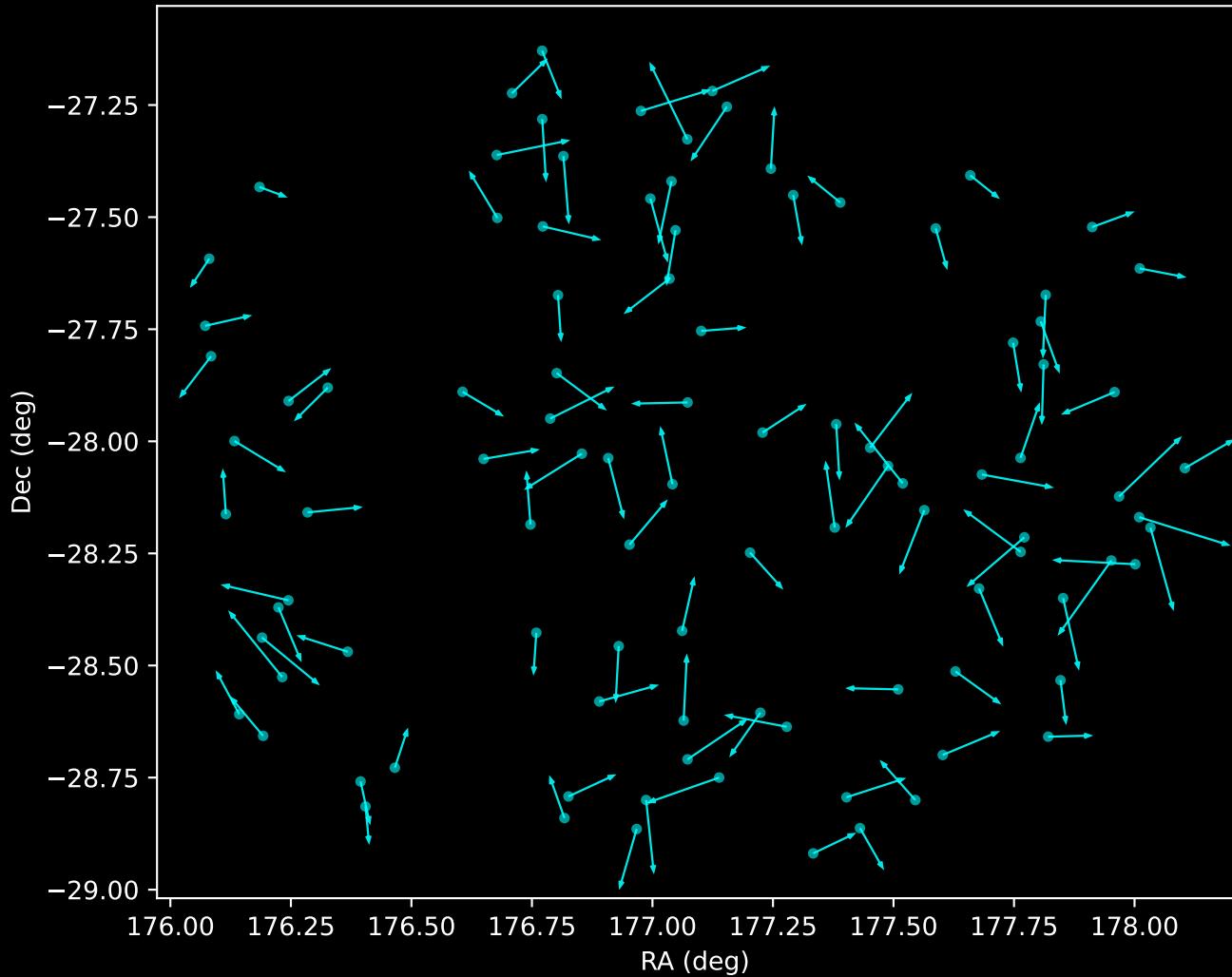
GALAH DR4 Noise Stream Proper Motion Vectors (n=100)
