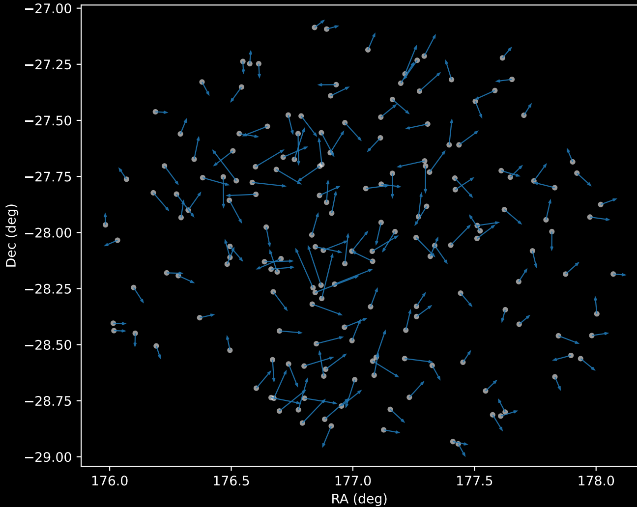
GALAH DR4 Cluster 0 Proper Motion Vectors (n=175)
