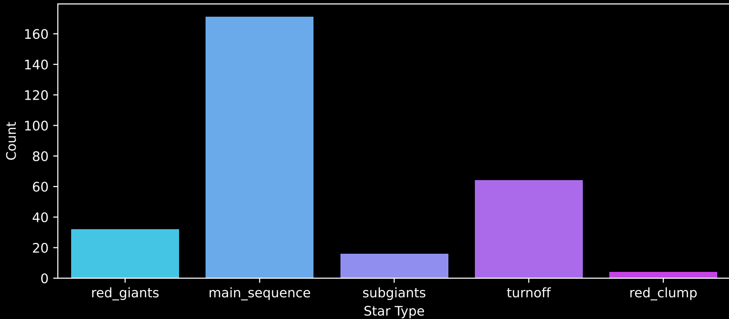
GALAH DR4 Field: [647] Count plot of Star Type
